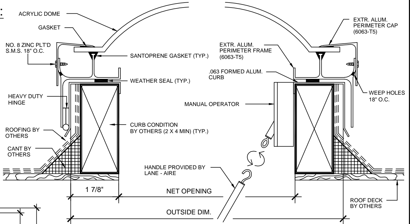
SECTION A - A SCALE : 1/2" = 1"
